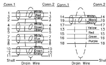
Pin Assignment
