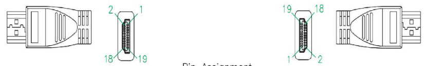
Pin Assignment
