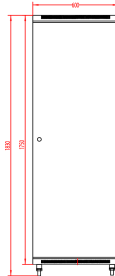
REAR DOOR
